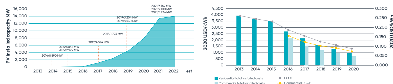
Figure 6. Solar PV expansion and LCOE reduction in Brazil.
