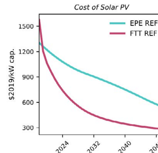
Figure 17. Cost of solar PV panels over time.
