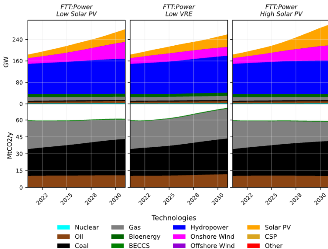
Figure 18. Power generation capacity and CO 2 emissions by technology in alternative scenarios using FTT.
