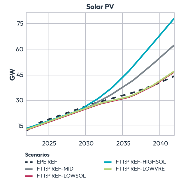
Figure 2. Power generation capacities of solar PV power for all scenarios in both cost-optimising (see EPE Ref) and new economic models (FTT scenarios).
