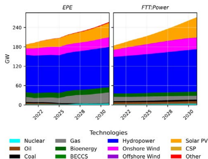
Figure 16. Baseline comparison for the energy mix between FTT and the IDM+4MD models until 2031.
