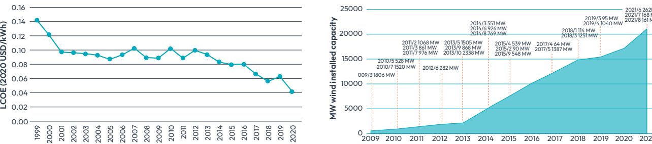
Figure 5. Onshore wind power expansion and LCOE reduction in Brazil.
